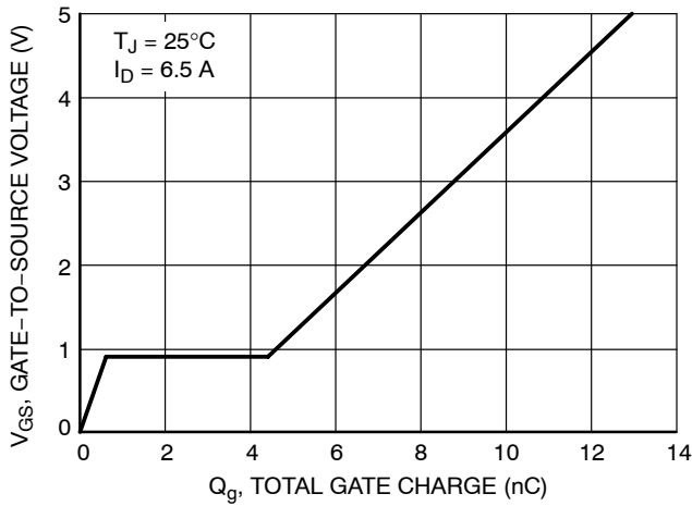
Figure 7. Gate-to-Source
